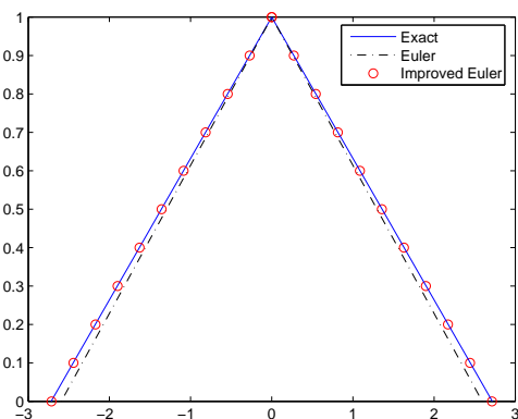
Figure 1: Solution for h=0.1
