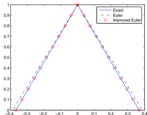
Figure 2: Solution for h=0.1
