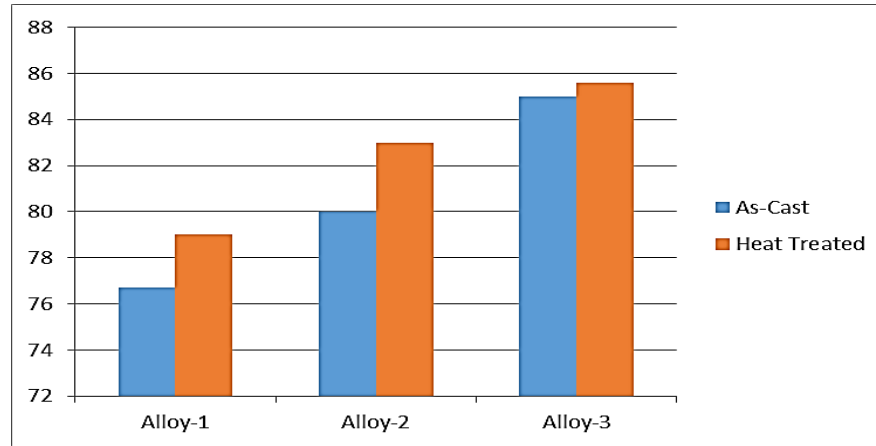
Fig. 5: Microhardness of as cast and aged Cu-5%Zn alloys with varying Ni content
