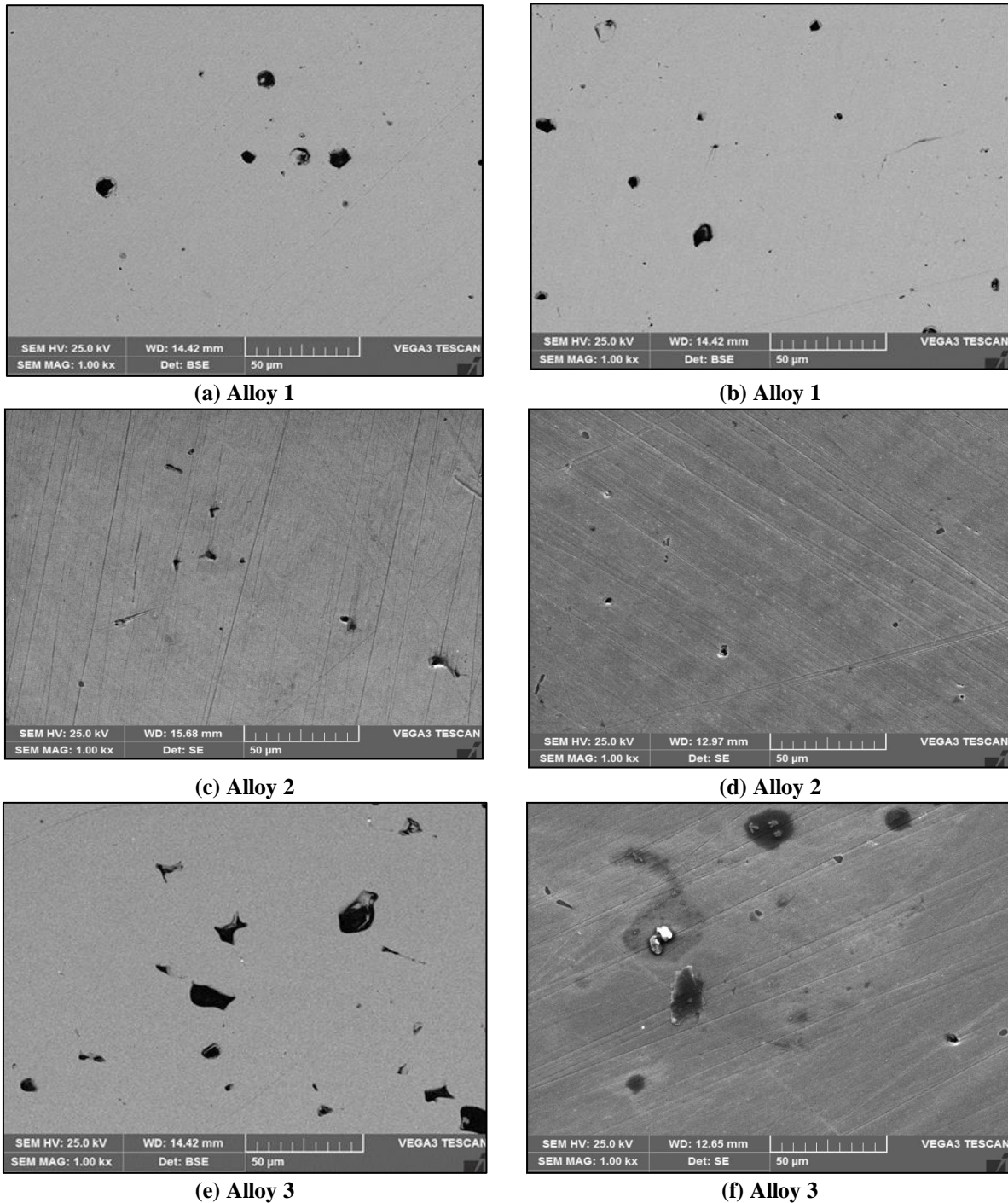
Fig. 3: SEM micrographs of (a,c,e) cast and (b,d,f) aged samples (4 hours)
