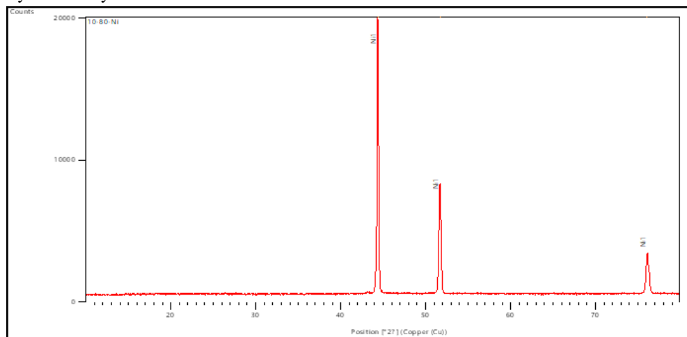
Fig. 1: X-ray diffraction patterns of as received Ni
