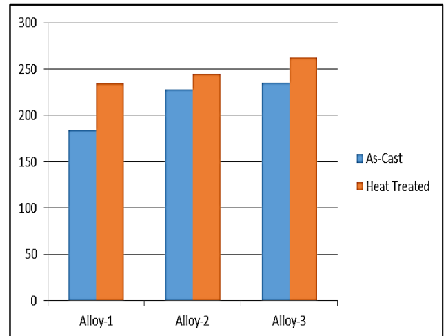
(b) Ultimate tensile strength
