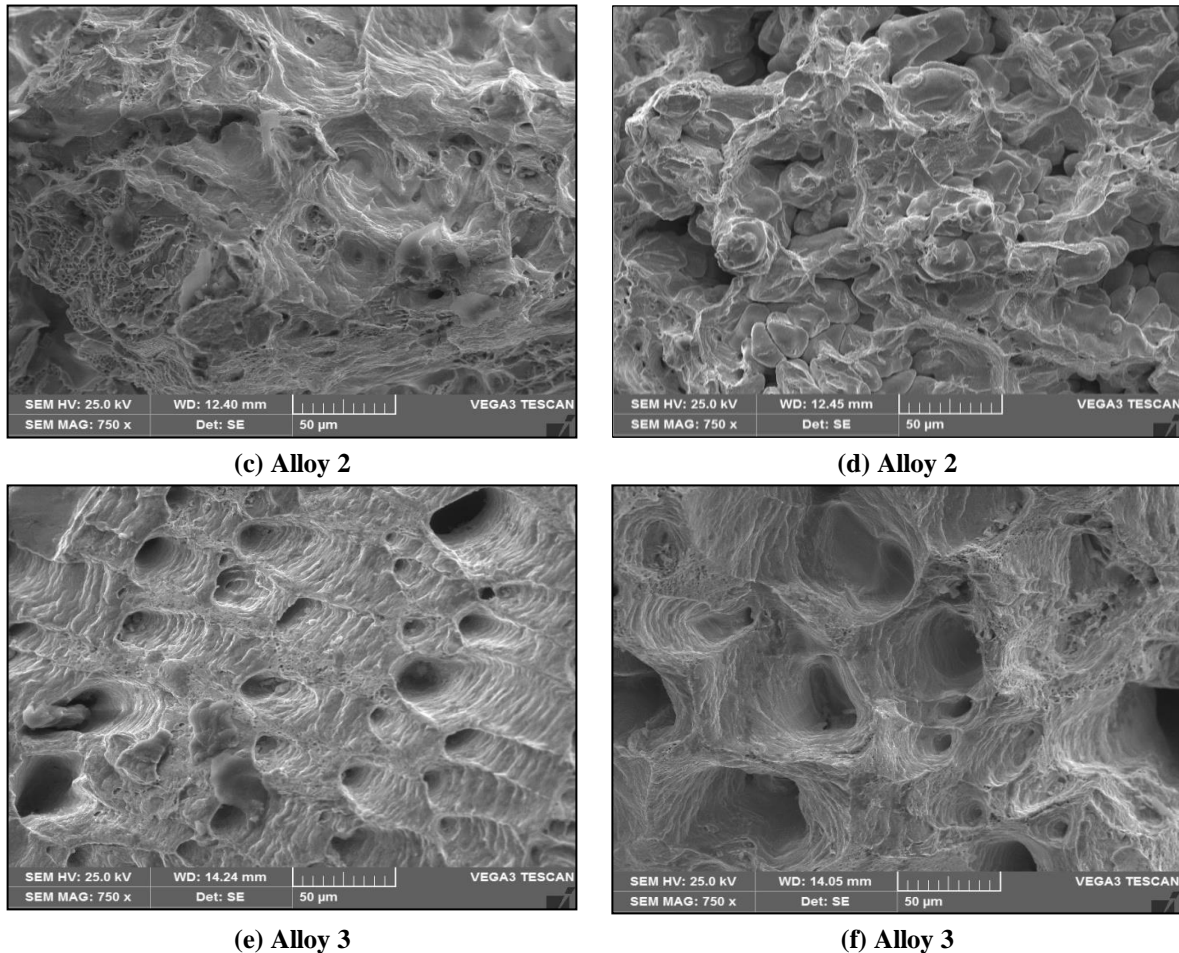
Fig. 7: SEM micrographs showing tensile fracture surface of (a,c,e) cast and (b,d,f) aged samples (4 hours)
