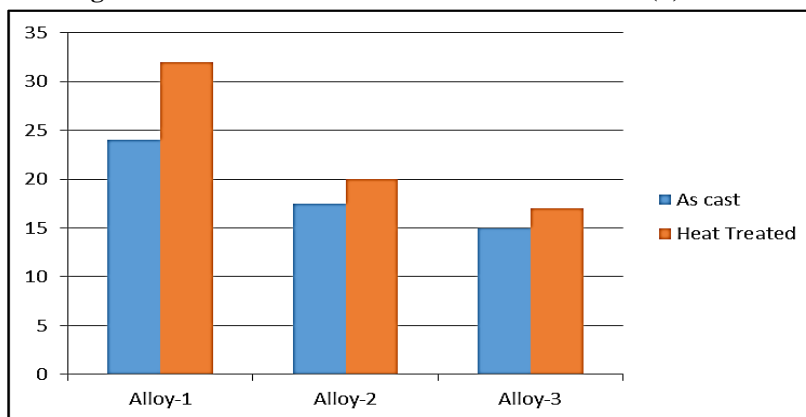
(c) Elongation at break
