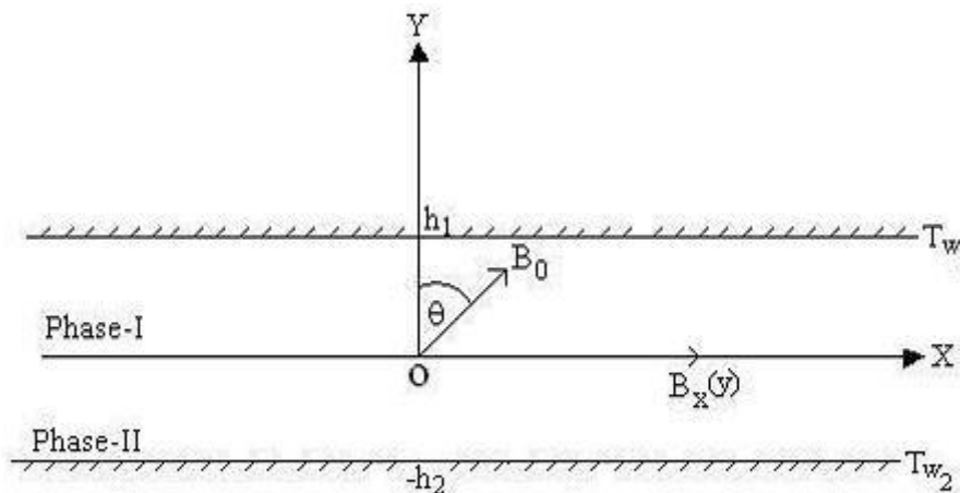
Fig 1: Physical Configuration
