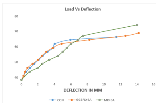
Fig. 7: Load deflection curves
