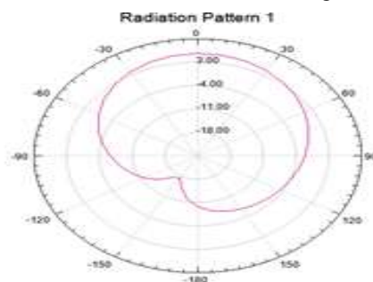
Figure 8. Experimental polarization graph
