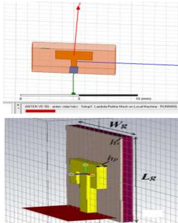
Figure 6. Sample rectangular microstrip antenna designed on HFSS software
