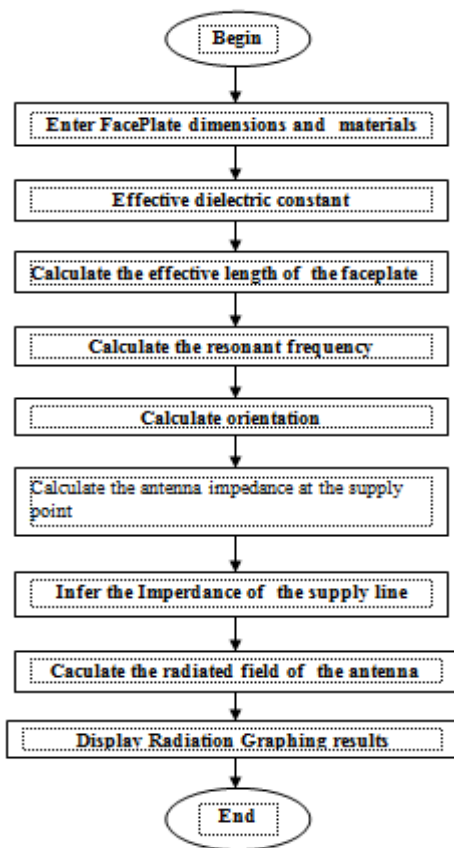
Algorithm flowchart of simulation program
