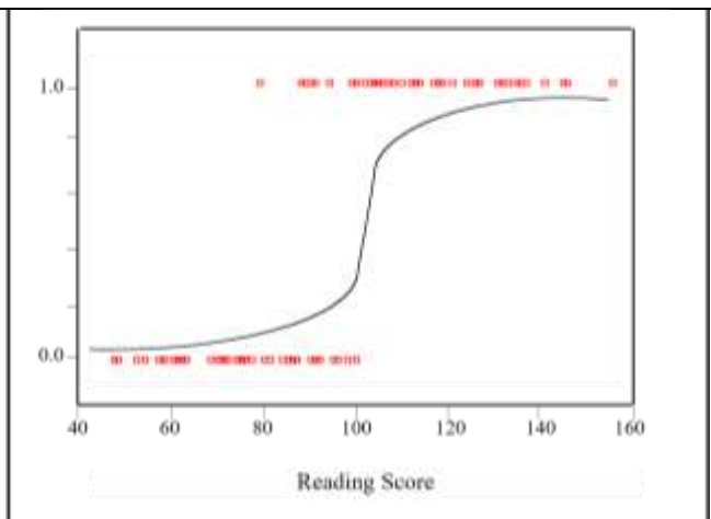
Figure 2. Relationship of a dichotomous outcome variable Y (1= Remedial Reading Recommended, 0= Remedial Reading Not Recommended) With a Continuous Predictor, Reading Scores
