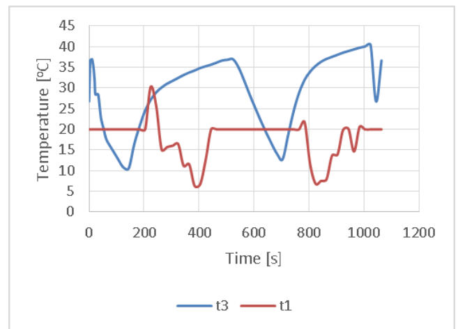
FIG 9. TEMPERATURE AT THE INLET OF THE COMPRESSOR, AND THE OUT LET OF THE CONDENSER
