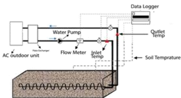
FIG. 2. SCHEMATIC DIAGRAM OF EXPERIMENTAL UNIT
