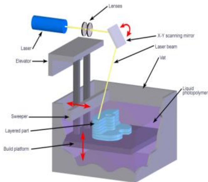
Fig. 5. Stereolithography
