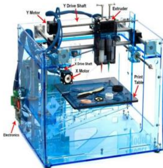
Fig. 1. 3D-printer
