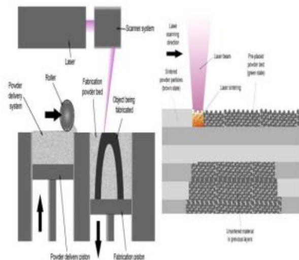
Fig. 3. Selective laser sintering
