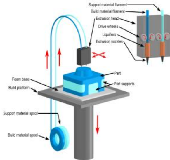
Fig. 4. Fused deposition modelling
