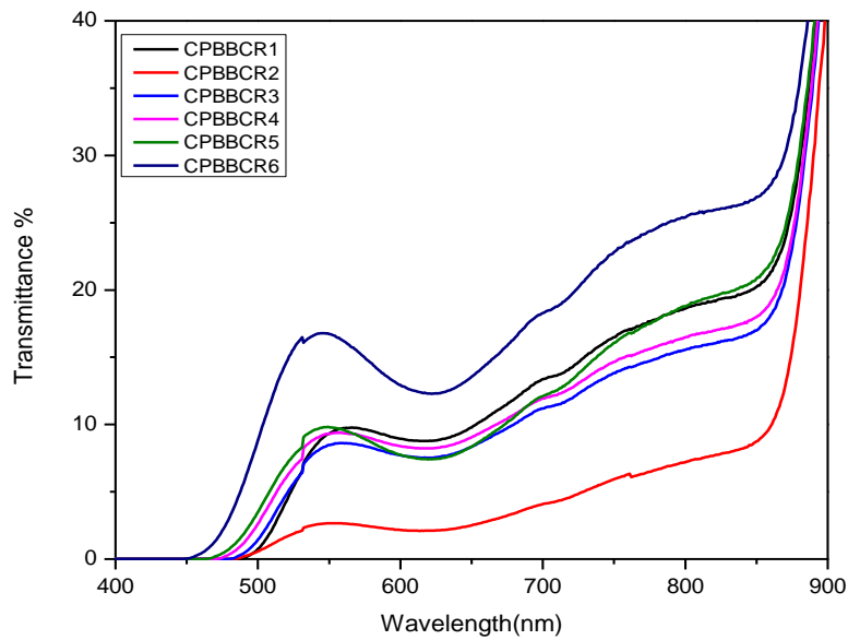
Figure 3: Optical transmittance spectra of CPBB CR glasses
