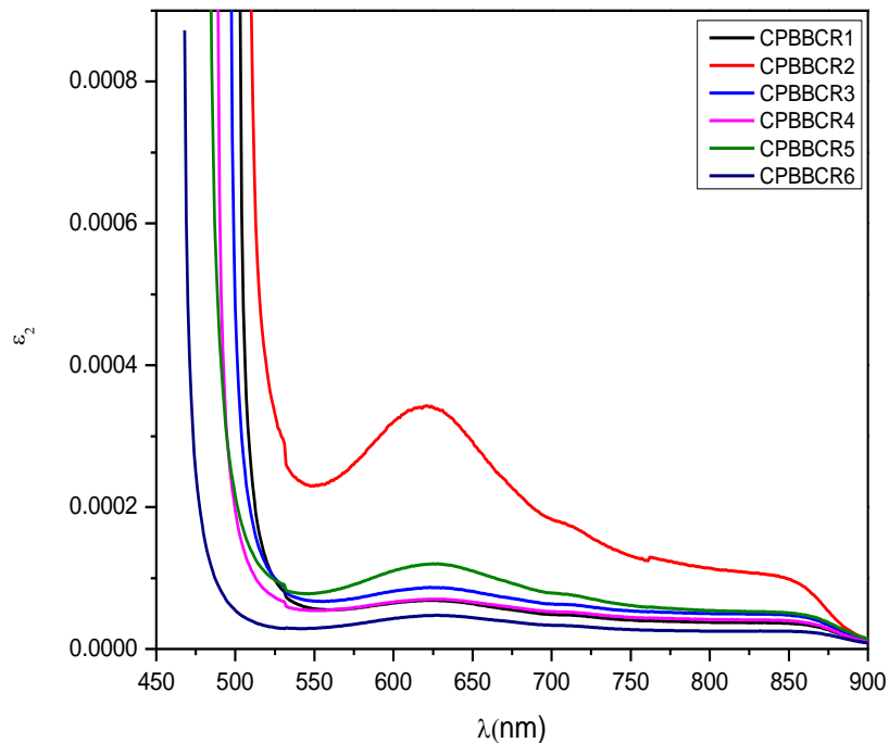
Figure 7: Imaginary part of the dielectric constant as a function of wavelength in CPBB CR glass system.
