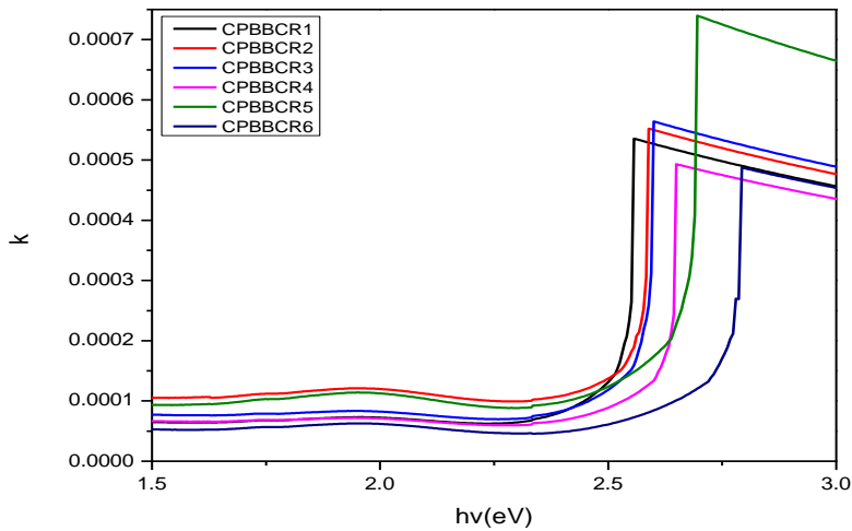
Figure 4: Extinction coefficient vs incident photon energy plot of CPBBCCR glasses
