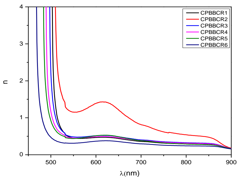
Figure 5: Refractive index vs wavelength plot of CPBBCCR glasses
