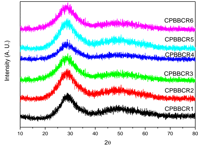
Figure 1: X-ray diffractogram of CPBBCR glass system [4]
