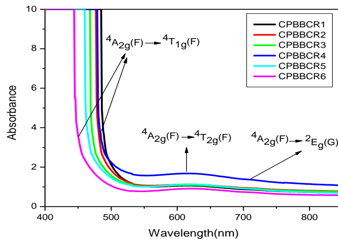
Figure 2: Absorbance vs Wavelength spectra of CPBBCR glasses [4]
