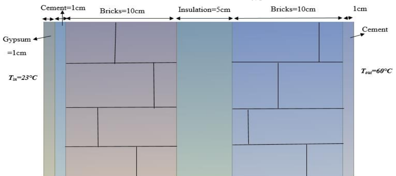
Fig. (1) Schematic diagram of the wall with thermal insulation to the middle of the wall.
