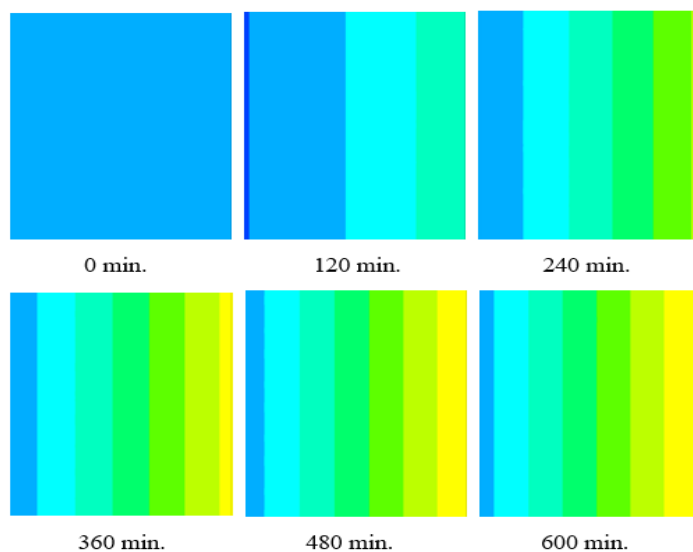
Fig. (4) Heat transfer stages inside the thermal insulation (Fibreglass).
