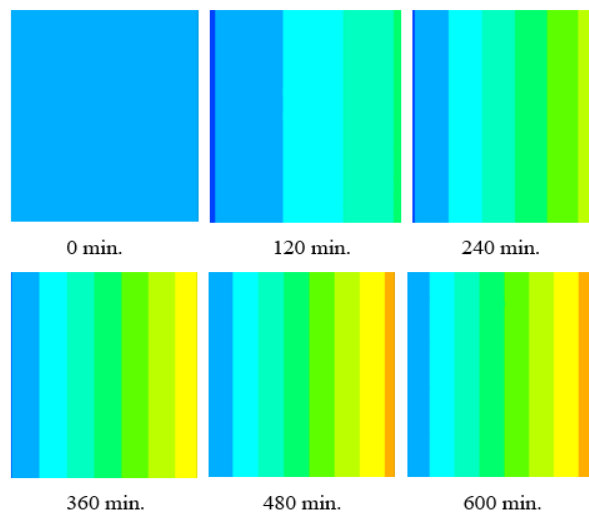
Fig. (3) Heat transfer stages inside the thermal insulation (Cellulose).
