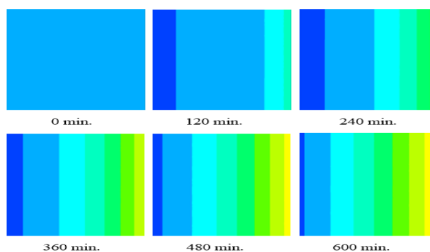
Fig. (7) Heat transfer stages inside the thermal insulation (Polyurethane foam).
