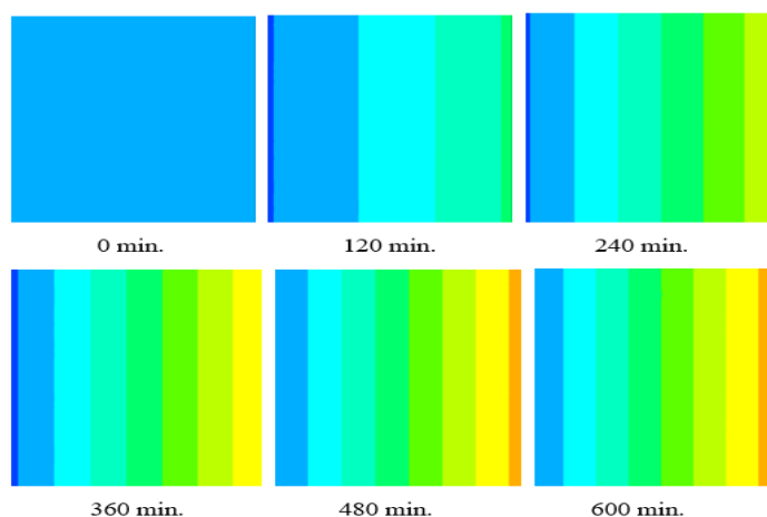
Fig. (5) Heat transfer stages inside the thermal insulation (Mineral wool).
