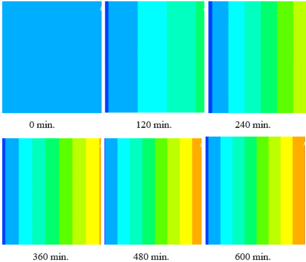
Fig. (2) Heat transfer stages inside the thermal insulation (air).
