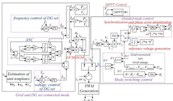
Fig. Unified control of the VSC for standalone and grid and DG set connected mode”.
