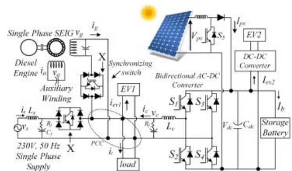
Fig. Topology of a CS.
