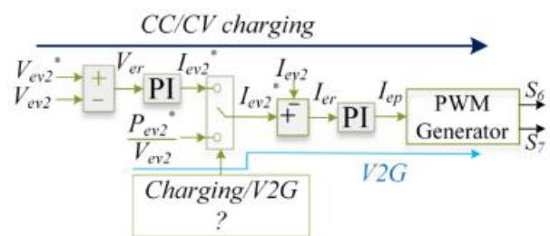
Fig.. “EV2 control for CC/CV charging and V2G power transfer”.
